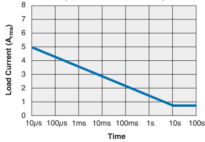
CPC1926Y Energy Rating Curve (Free air, no heat sink)
