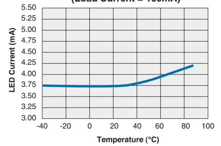
CPC1926Y Typical I F for Switch Operation vs. Temperature (Load Current = 100mA)
