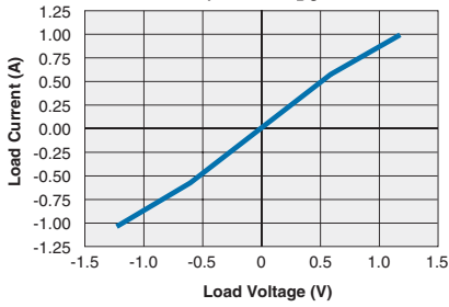
CPC1926Y Typical Load Current vs. Load Voltage (Ambient Temperature = 25°C) I F = 10mA DC
