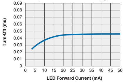
CPC1926Y Typical Turn-Off vs. LED Forward Current (Load Current = 100 mA DC )
