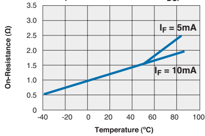
CPC1926Y Typical On-Resistance vs. Temperature (Load Current = 100 mA DC )
